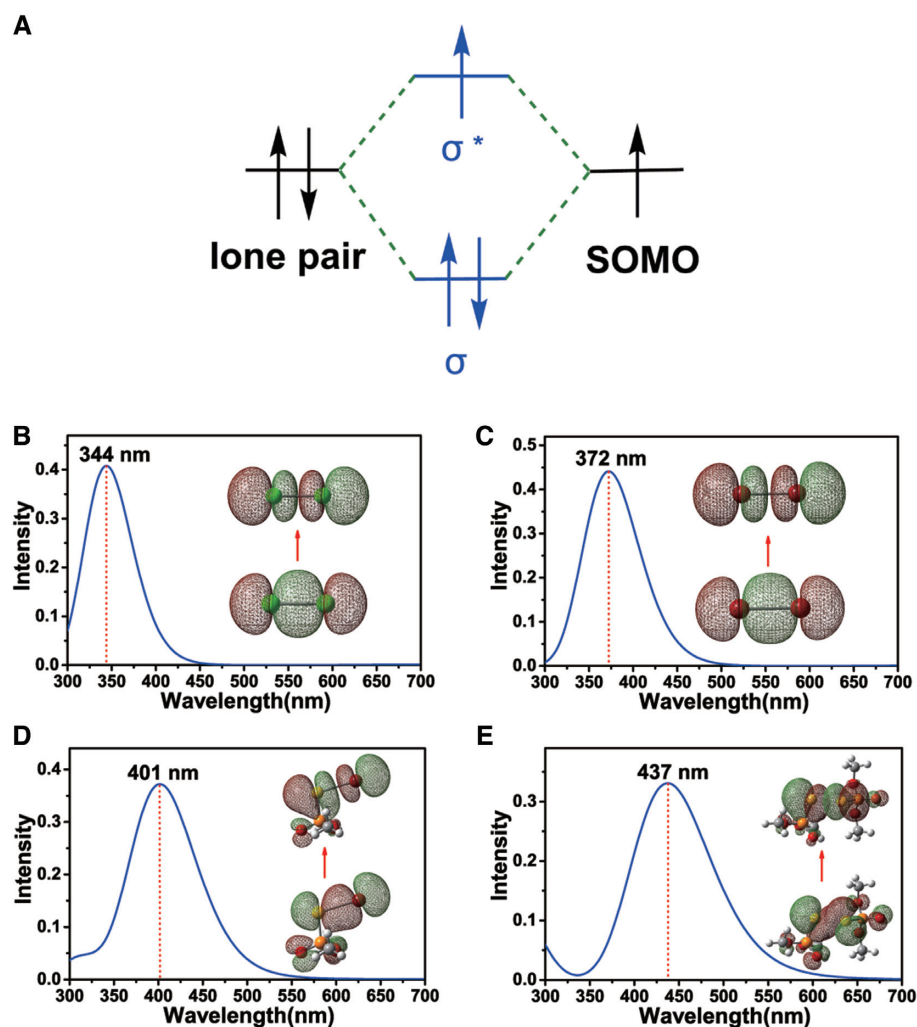
Figure 4. (A) Simplified MO energy levels for the hemi-bonded species. Calculated absorption spectra of (B) Cl 2 -• , (C) Br 2 -• , (D) -P-S:•Cl and (E) -P-S:•S-P-. MOs dominantly contributing to the optical transition are also shown. Chlorine, bromine, carbon, oxygen, sulfur, phosphorus and hydrogen atoms are denoted with green, vermeil, gray, red, yellow, orange and white spheres, respectively.
