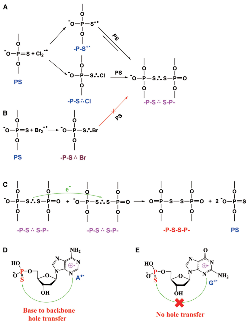
Figure 3. Schematic elementary oxidation mechanisms of PS in free model ( O,O -diethyl thiophosphate) and PS in oligomers ( O,O -dinucleoside thiophosphate) by (A) \text{Cl}_2^{\bullet-} (strong oxidant radical) and (B) \text{Br}_2^{\bullet-} (mild oxidant radical). (C) Proposed reaction scheme for the end-product -\text{P}-\text{S}-\text{S}-\text{P}- formation via the radical-radical recombination of -\text{P}-\text{S}^{\bullet}\cdot\text{S}-\text{P}- . Possible hole transfer processes (D) from \text{A}^{\bullet+} to PS or (E) from \text{G}^{\bullet+} to PS.
